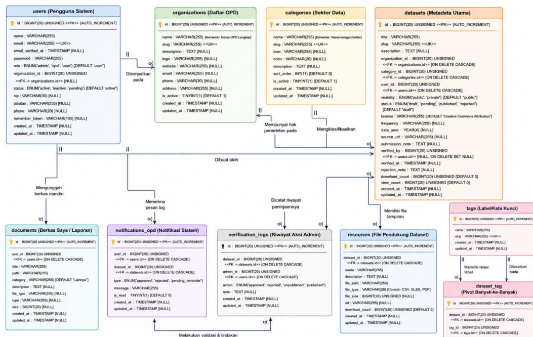
Gambar.D. Entity Relationship Diagram (ERD)
