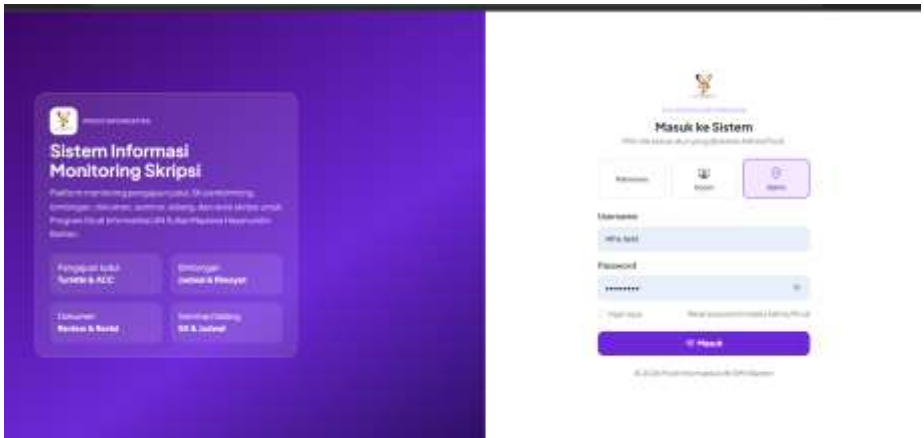
Gambar 3. Login Admin
